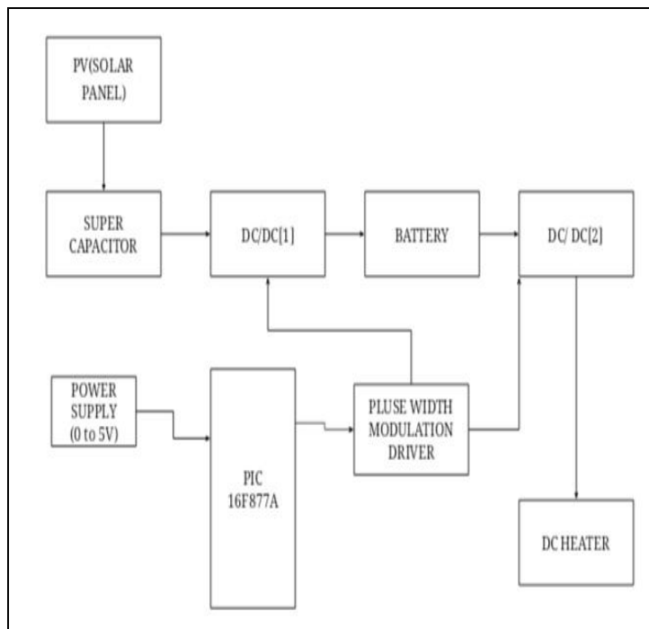
Figure 2 Block Diagram
